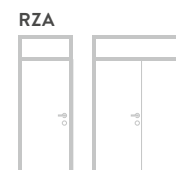
RZA Ceiling height frame with head, transom and fan light up to a clear frame height of 2,520 mm (single leaf, double leaf)
