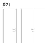
RZI Ceiling height frame without head and transom up to a clear ceiling height of 2,600 mm (single leaf, double leaf)
