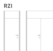
RZI Ceiling height frame without head and transom, with top panel up to a clear ceiling height of 2,600 mm (single leaf, double leaf)
