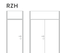
RZH Ceiling-height frame without cross rail, with transom and fanlight up to a ceiling height of 2,600 mm (single leaf, double leaf)
